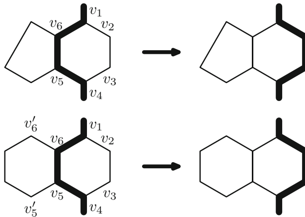
Fig. 5 Configurations analyzed in the proof of Lemma 4
